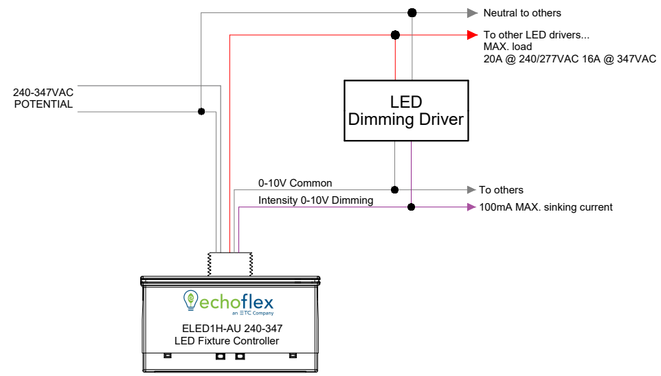
Typical Classroom w/Daylight Harvesting
